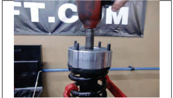
Install new assembled strut extension and tighten to spec.
