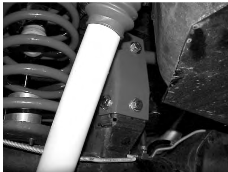
Rear Trackbar Bracket (installed) driver side view
