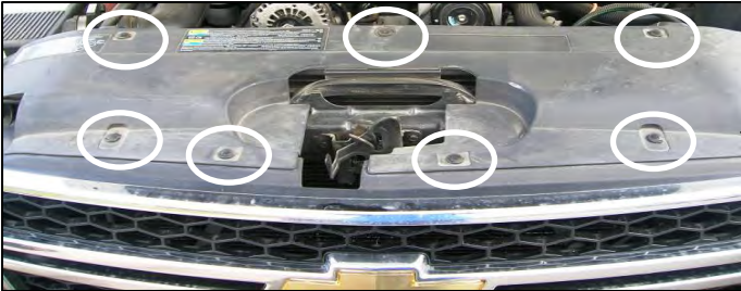
Figure 2 – Remove 7 factory plastic fasteners
