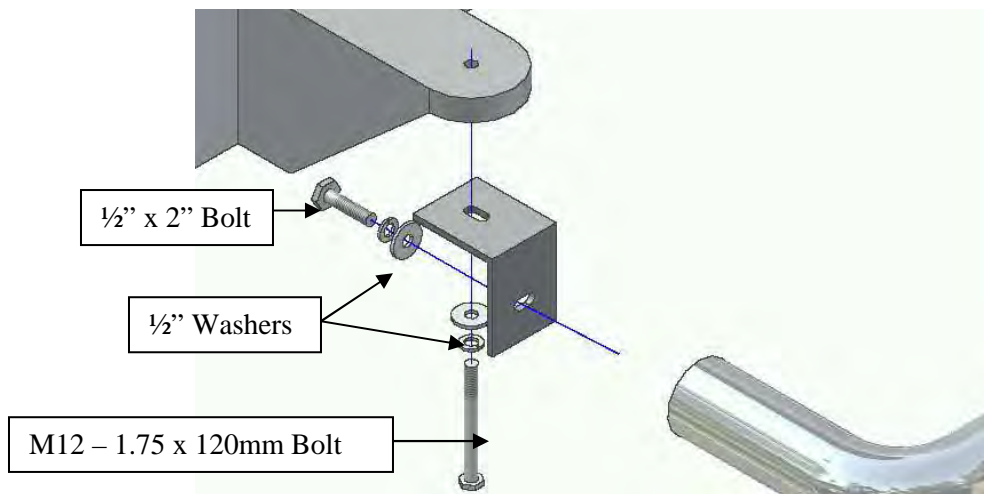
Figure 1.2 – Front Bracket
