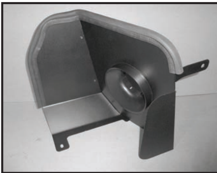
Step 10 Assemble the heat shield with the tabs placed on the outside of heat shield. Install the rubber bulb seal. Place the velocity stack adaptor in the heat shield and fasten it securely to the heat shield with the supplied hardware.
