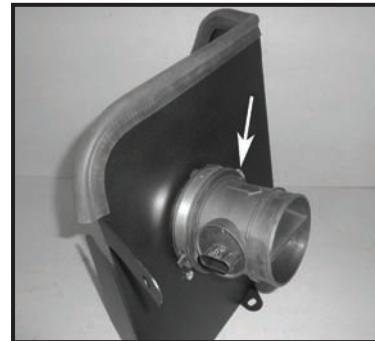
Step 11 Install the MAFS on the end of the velocity stack adaptor. Take note of the orientation of the MAFS and once in the desired location fasten it securely.
