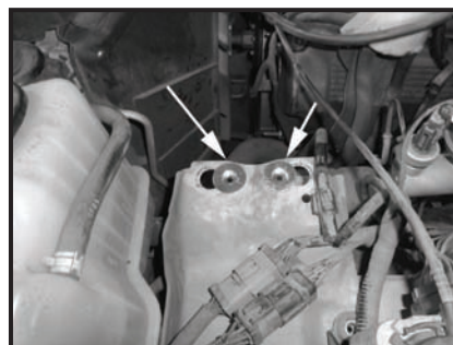
Step 14 Install the heat shield upper mounting spacers as shown.
