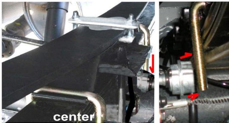
install hardware clear of factory sensor at axle rear
