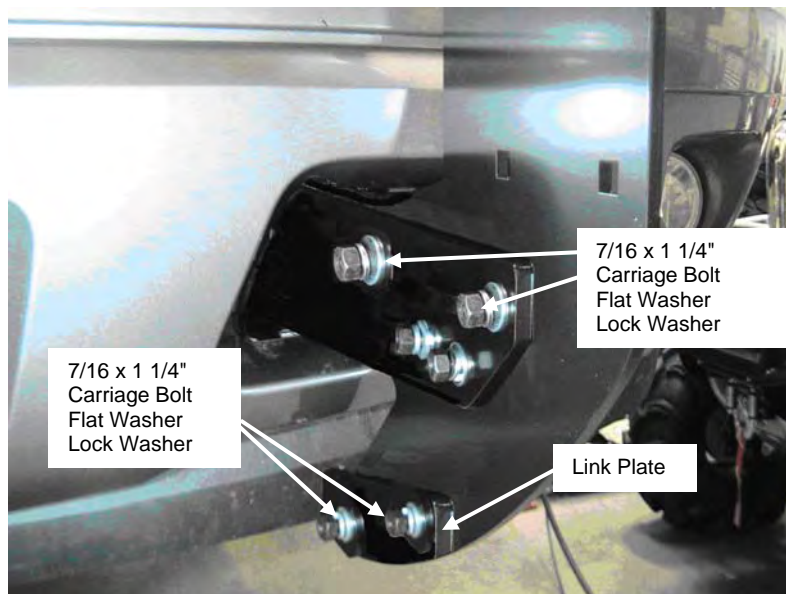
Figure 5. Mounting Side Member. (Suburban link plate will differ slightly)
