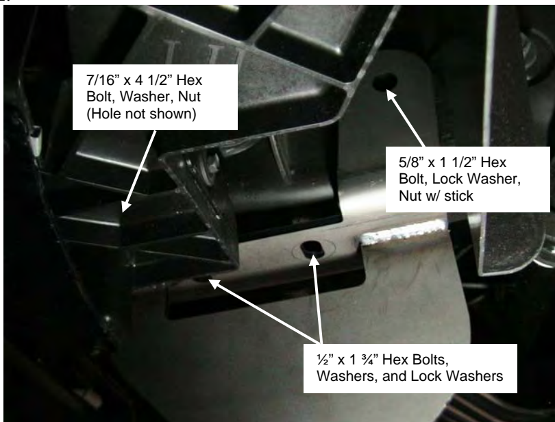
Figure 2 Placement of the Frame Bracket (Driver Side Outboard Shown)
