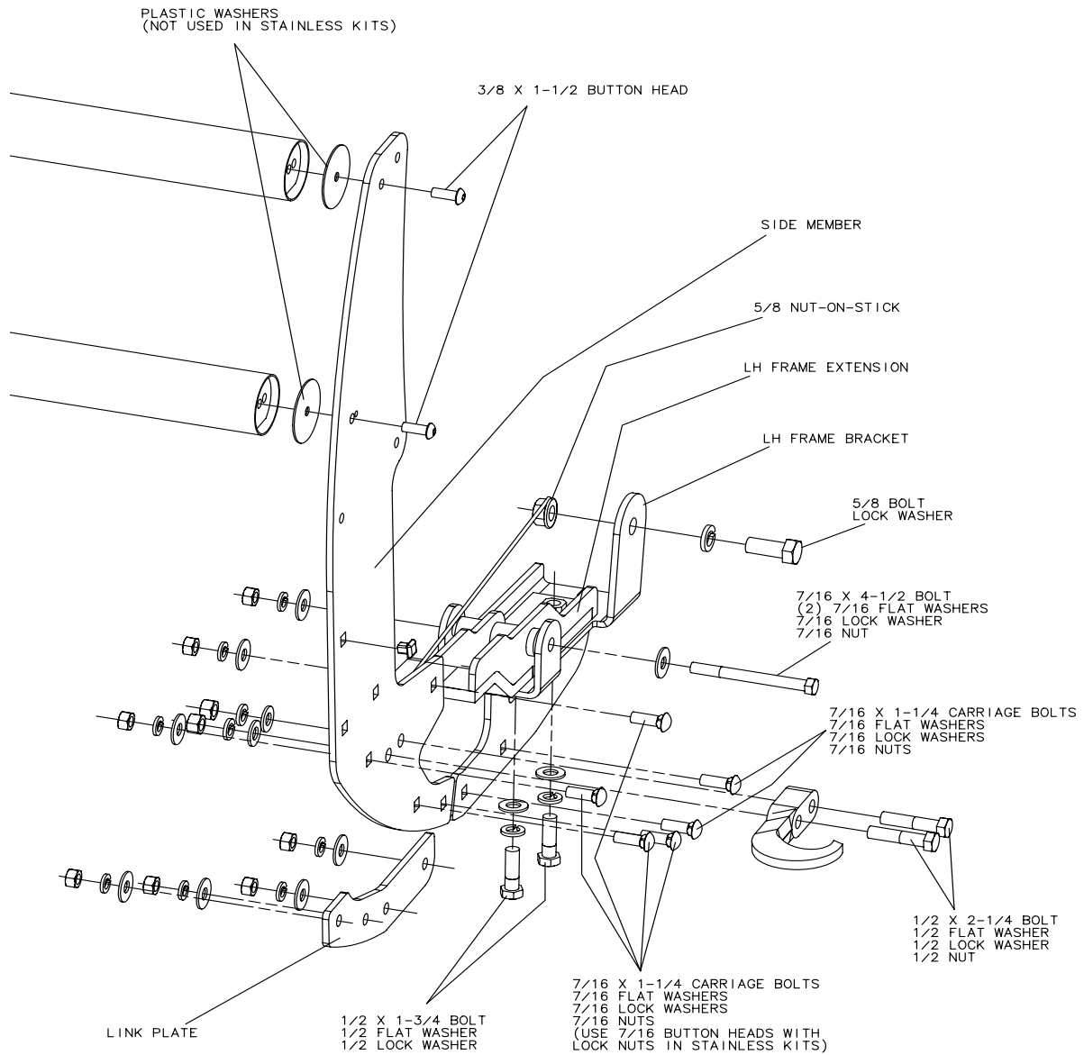
Figure A. Exploded View
