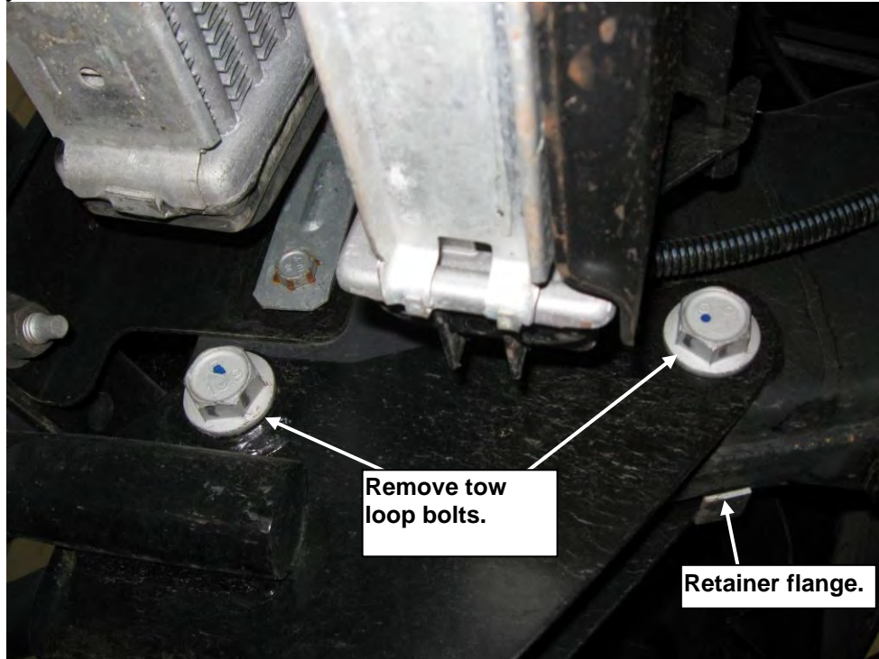
Figure AA Bolts attaching tow loops to frame (viewed from center of vehicle, looking outward)
