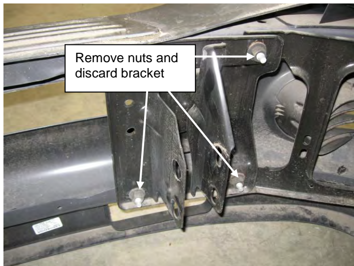
Figure DD OEM bumper bracket removal.
