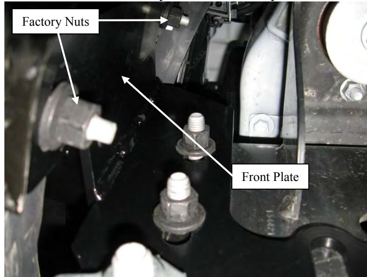
Figure 2: Bolts attaching Frame Extension Bracket to bumper (viewed from center of vehicle, looking outward)
