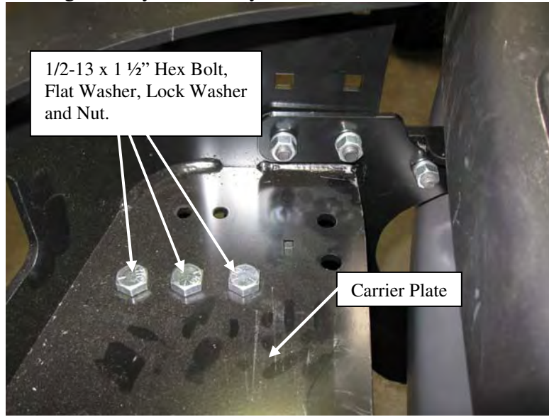
Figure 7: Large Frame Carrier: Carrier Plate Hex Bolt Positions.
