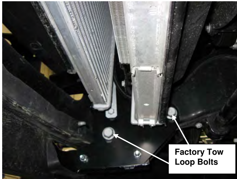
Figure 1: Bolts attaching Frame Extension Bracket to frame (viewed from center of vehicle, looking outward)
