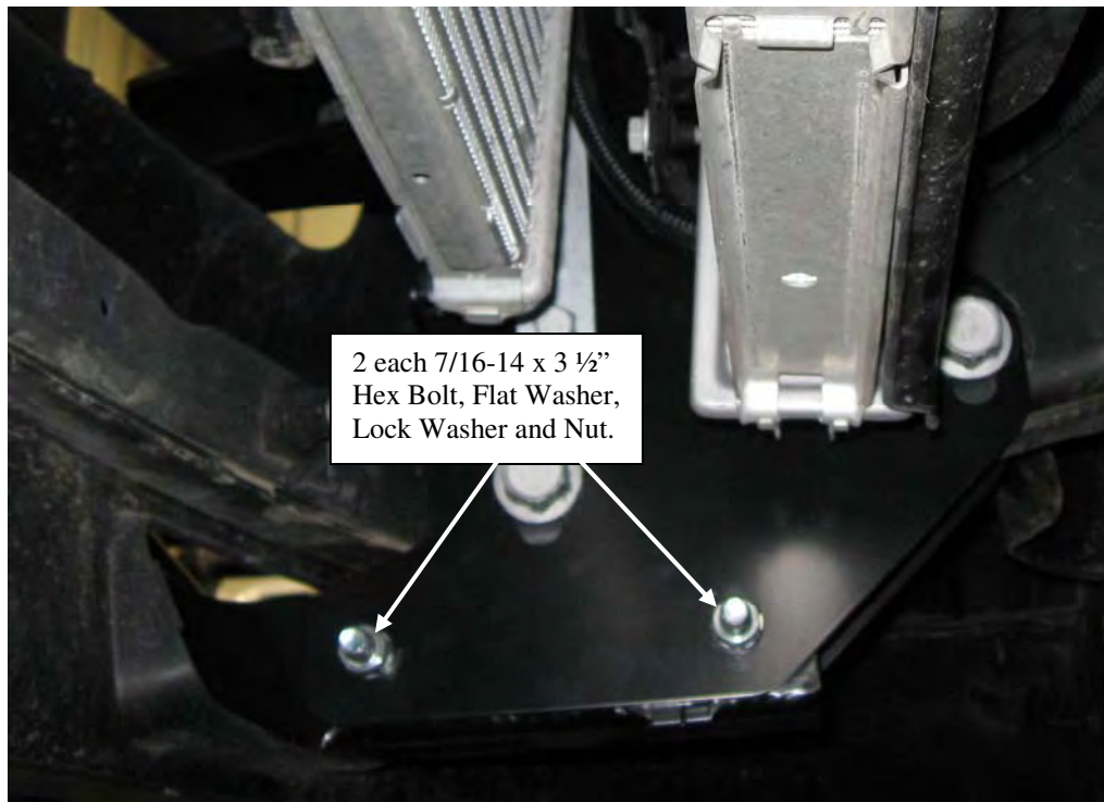
Figure 5: Large Frame Carrier: Lower bolt position.
