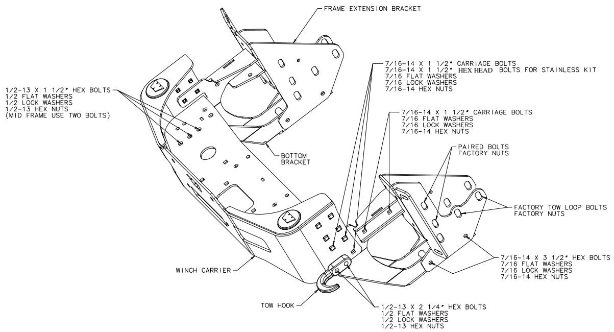
Figure A: Large Frame Fastener Placement (Mid Frame Not Shown Fastener Placement the Same Except as Noted)
