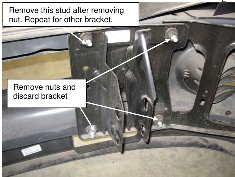
Figure DD OEM bumper bracket removal.
