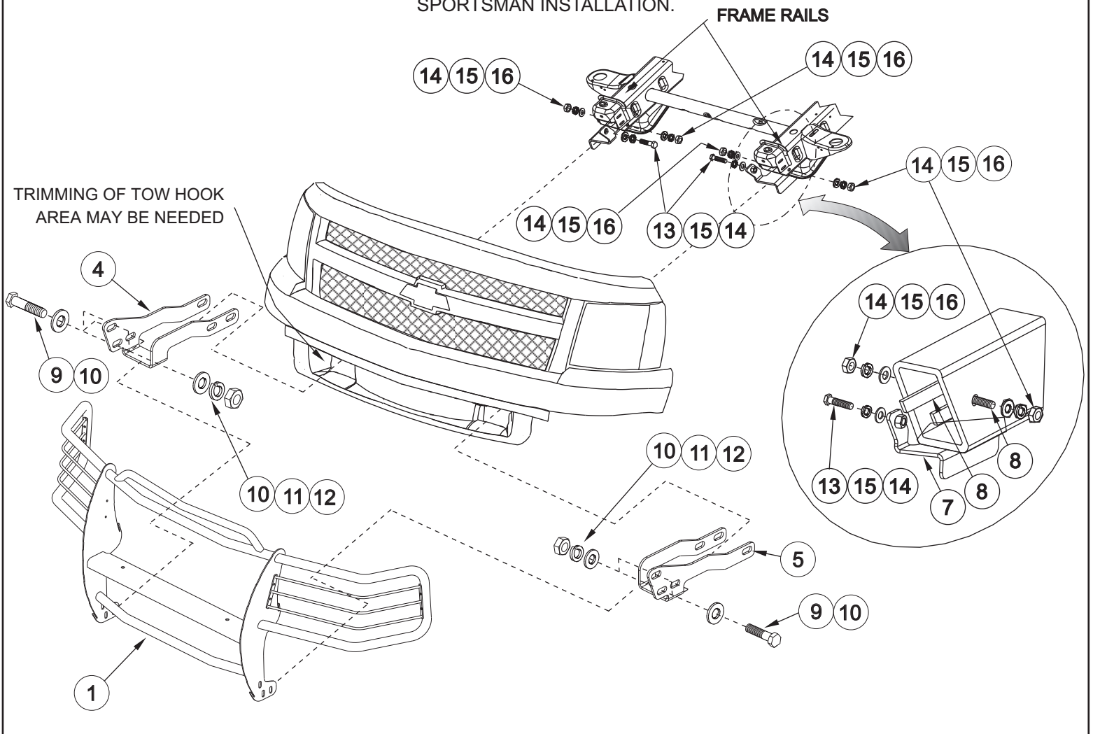
FIGURE 5 SPORTSMAN INSTALLATION.
