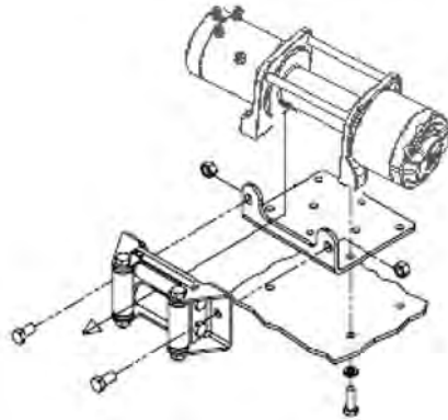
Installation Drawings
