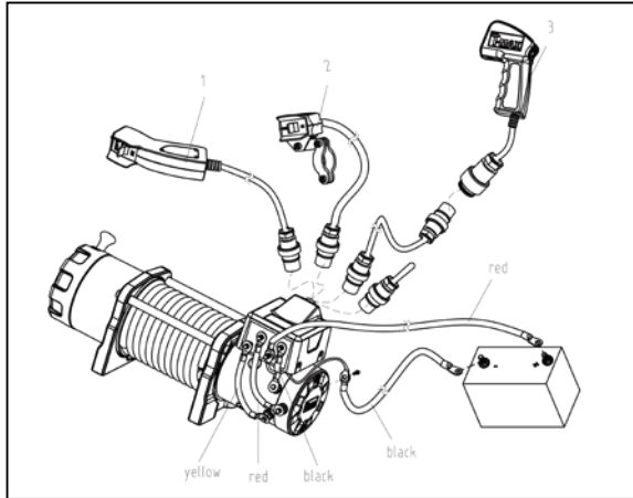
Battery Cable Wiring Diagram
