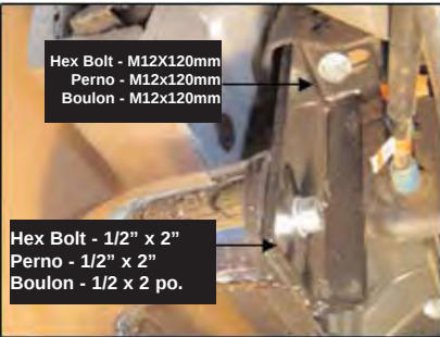
Rear Bracket (Fig. 1) Soporte trasero (Fig. 1) Support arrière (fig. 1)
