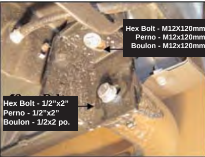
Front Bracket (Fig. 3) Soporte delantero (Fig. 3) Support avant (fig. 3)
