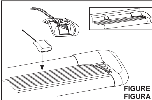
FIGURE 1 FRONT DRIVER SIDE SHOWN FIGURA 1 LADO DEL CONDUCTOR DELANTERO COTE CONDUCTEUR DEVANT
