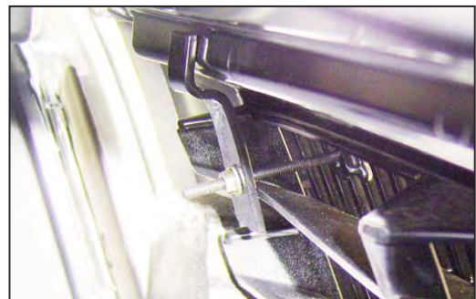
FIGURE 2 - Bent Brackets (4) - Top
