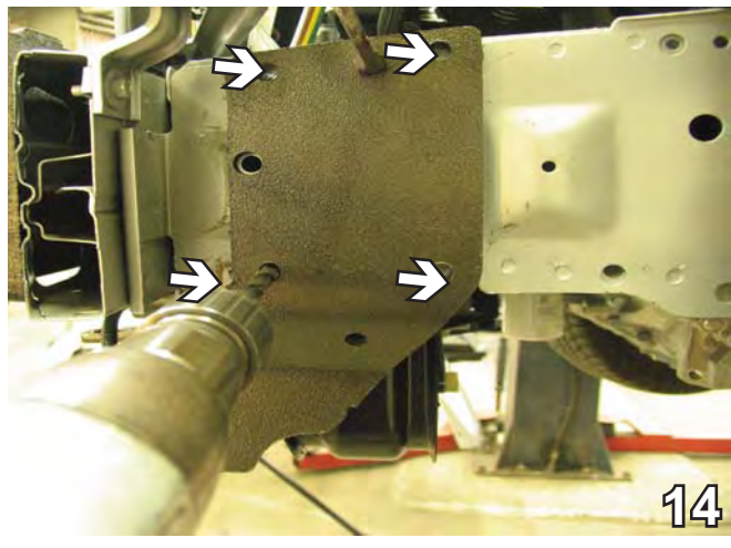
14. Using the baseplate as a template, drill four corner holes into the frame webbing with the 13/32" drill bit. Insert 3/8"-16 x 1 1/4" hex bolts into holes and tighten to the 1/4" lock washers and 3/8-16 hex nuts.
