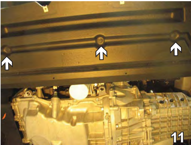
11. Using the flat screwdriver, remove three pushpins on the bottom and remove the black plastic piece. Set pushpins and plastic aside to be reinstalled later.
