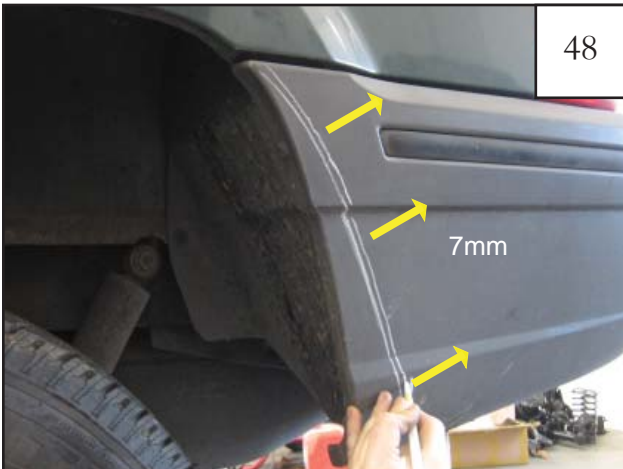
Trace a second line 7mm offset from previous line toward rear of vehicle.
