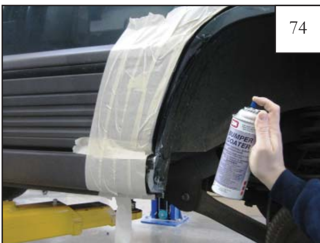
Using spray paint, repaint the sanded edge of the wheel well.
