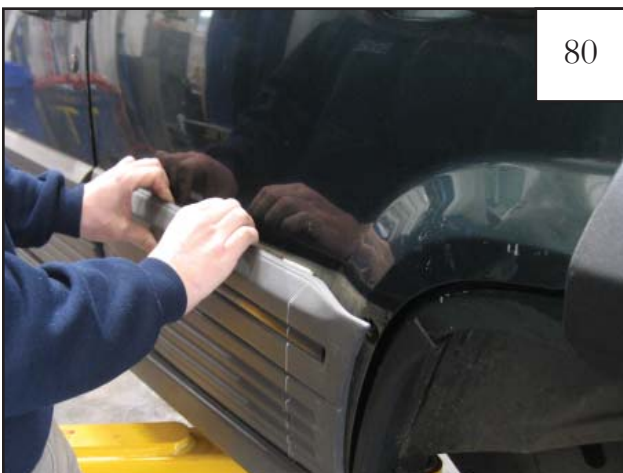
Remove the body side cladding from the vehicle. First, lift up by top edge to release top of cladding. Then pull bottom of cladding straight out from side of vehicle.
