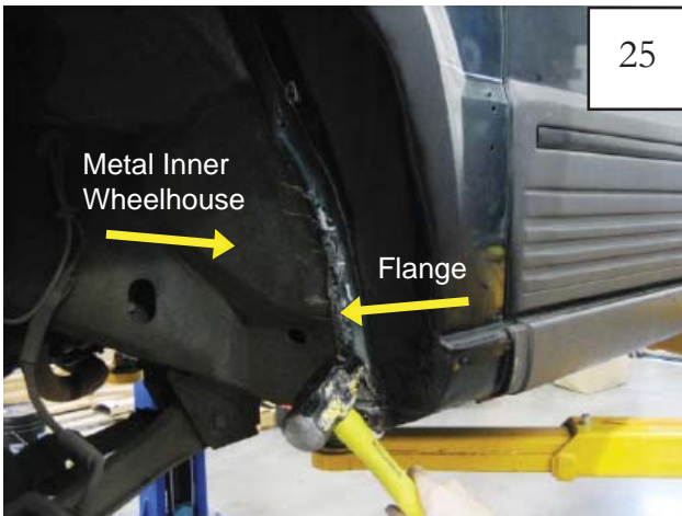
25 Pound the fender flange back over to match the face of the metal inner wheel house with a heavy hammer.
