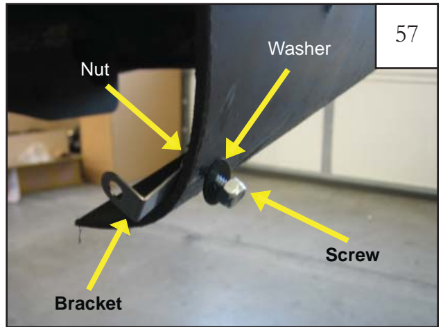
Start a washer, screw, and nut combination through the two holes and brackets in the bumper.
