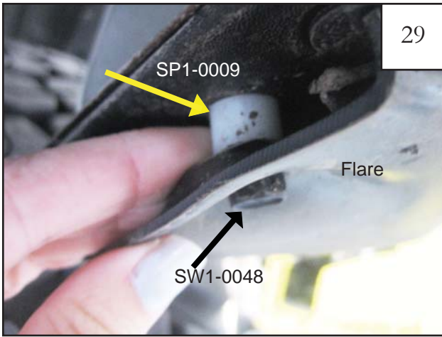
At lower REAR underside of flare, slip a supplied Spacer (SP1-0009) between flare and bumper (spacer is white in picture for visibility). Then install a supplied Bolt (SW1-0048) through hole in flare and spacer, and into bumper skin.
