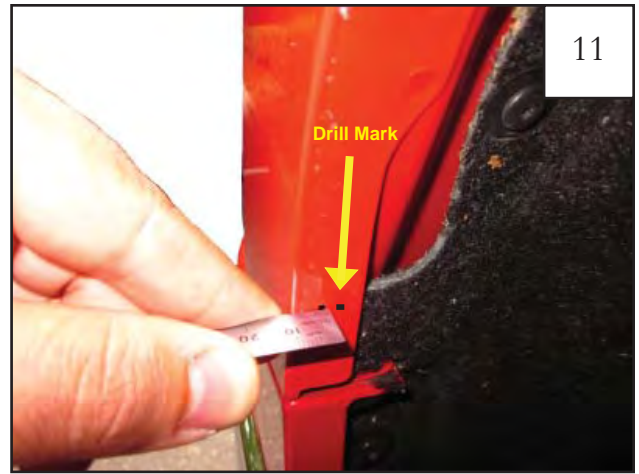
Remove the flare. Using the marks made in step 10 as a guide, measure inward from the outside edge of the fender to verify proper depth of original marked location. Mark must be minimum of 22mm in from outside edge of fender, if short, adjust marks to 22mm.
