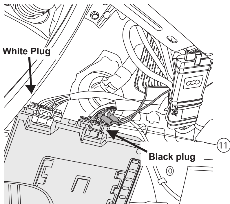
Powerstep Connection Module
