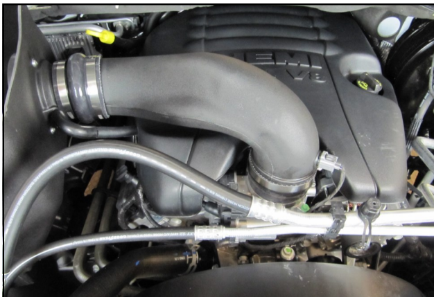
16. Install the Intake Tube, Hump Hose side first, onto the Cool Air Box, then onto the throttlebody. Align all four Clamps and tighten them. Reconnect the air temperature sensor.
