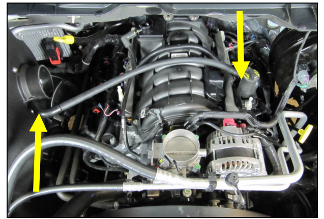
12. Install the Elbow side of the Airaid PCV line onto the Barbed Fitting on the Cool Air Box and connect the other side to the factory valve cover elbow.
