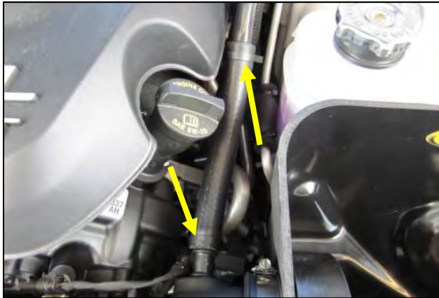
13. When equipped, secure the PCV Hose on both ends using the two Speed Clamps.
