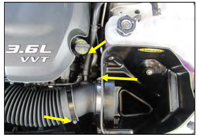
12. When equipped, slide the factory intake tube onto the Airaid Tube, adjust if necessary and tighten the Clamps. Connect the crank case breather line to the Barbed fitting using the supplied PCV Hose.
