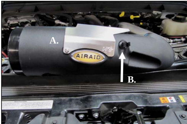
8. A.) Attach the Heat Shield to the Airaid Intake Tube as shown using three 1/4 -20 Button Head Bolts B.) Insert one Hose Anchor into the threaded insert in the Intake Tube. Apply the Airaid Badge to the tube as shown.
