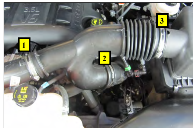
3. Loosen the three clamps on the intake tube and remove it from the vehicle.
