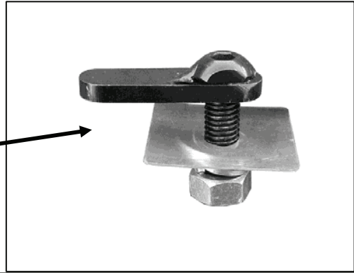
(Fig 5) Use M10 x 30mm Bolt Plate for passenger side inner location (same bolt plate used on center and rear brackets)
