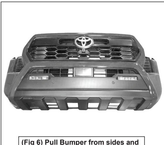
(Fig 6) Pull Bumper from sides and forward to detach from vehicle
