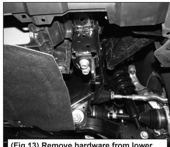
(Fig 13) Remove hardware from lower Frame Mounting Bracket mounting point
