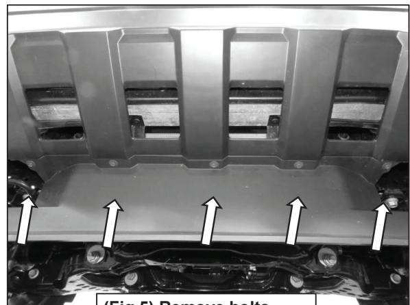
(Fig 5) Remove bolts from underneath bumper
