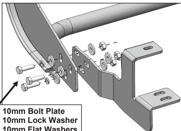
(Fig 16) Attach Grille Guard to Frame Mounting Bracket
