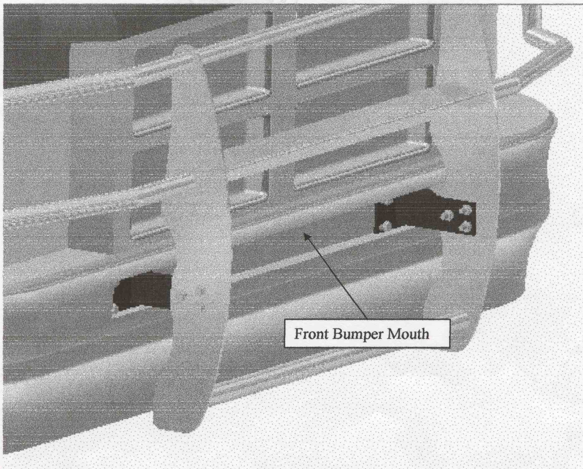
Figure 1.1 – Fully Assembled Grill Guard
