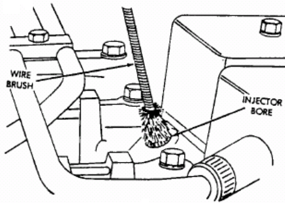
Fig 5: Cleaning Cylinder Head Injector Bore
