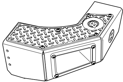
Bumper, Rear End Cap Assembly - Left Part #550.24 Qty. 1
