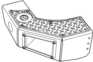
Bumper, Rear End Cap Assembly - Left Part #550.23 Qty. 1
