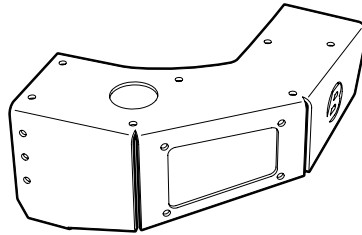
Rear Bumper End Cap - Right Part #522.24 Qty. 1
