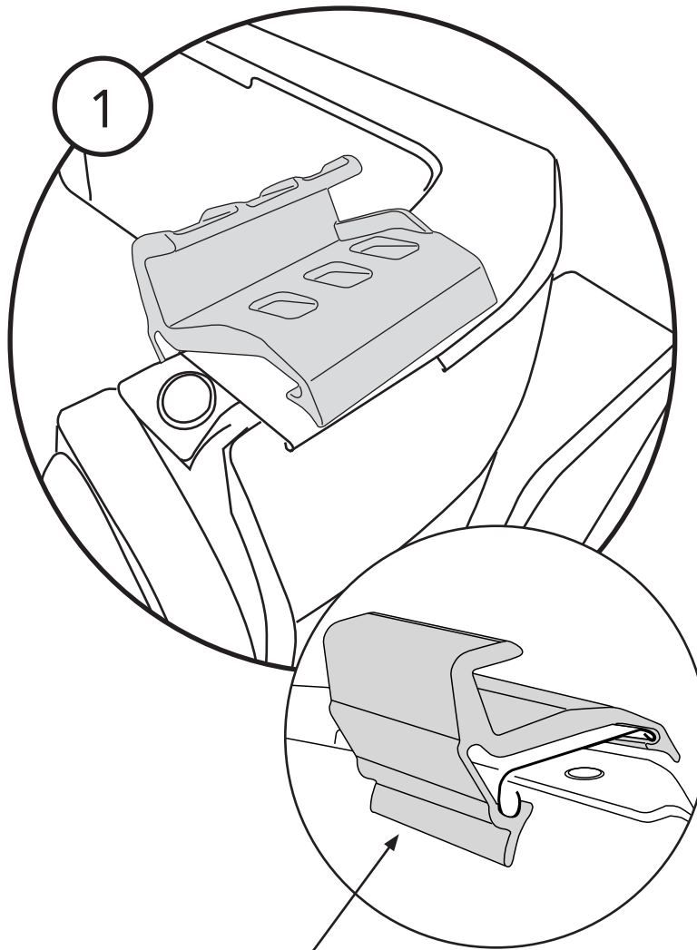
Tailgate Bar Mounts #539.56 - Right (shown) Qty. 1
