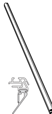
Rear Rail (55 inches) Part #581.85P Qty. 1
