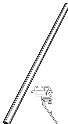
Front Rail (57.5 inches) Part #581.84P Qty. 1
