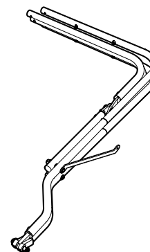
Bow Stack - Passenger Side Part #579.38 Qty.1
