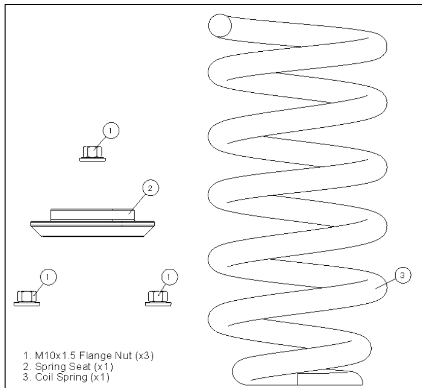
Fig 3: Bilstein supplied components
