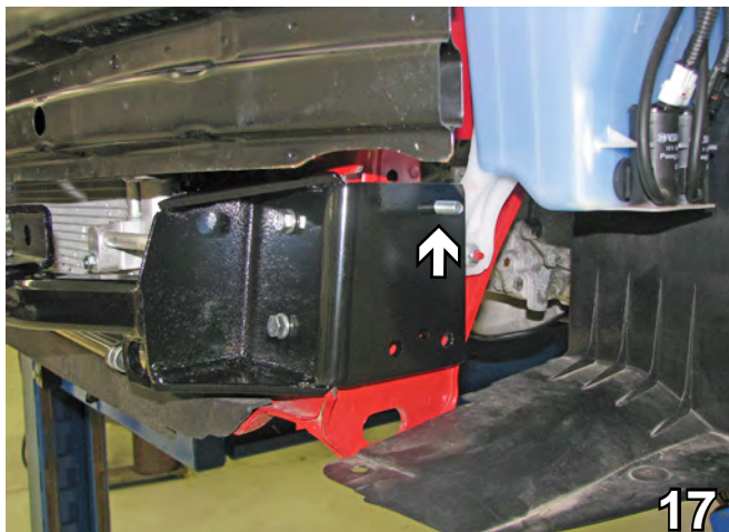
17. Align the baseplate with the upper existing hole on the side of the frame extension. Insert 3/8-16 x 2" hex bolt through baseplate's top hole and 3/4" spacer between the frame and the baseplate. Install 3/8" lock washer and 3/8-16 hex nut on the back side of webbing, tighten with loctite. On the driver side, the bolt comes through the frame to the outside of the baseplate. Be sure the baseplate is level with respect to the vehicle frame.
