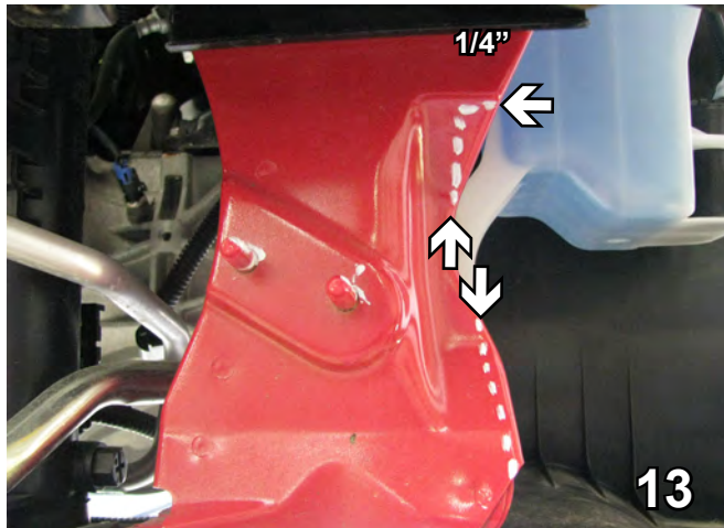
13. Cut 1/4" inch across where the frame starts to bow and straight down. Continuing on down trim off 1/4". Do this on both sides.
