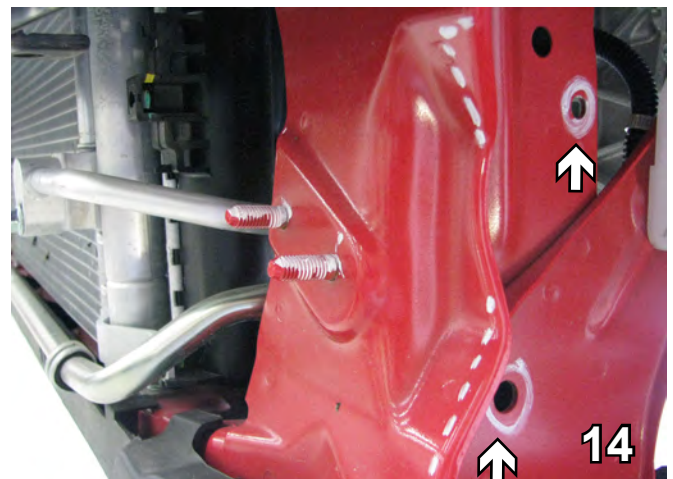
14. Locate these two existing holes on lower frame extension, just above tie down bracket and drill out with the 13/32" drill bit. Do this on both sides.
