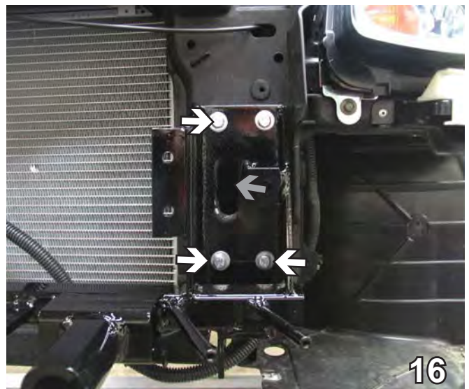
16. Insert the additional 8MM hex bolts, use Loctite Red and tighten according to specs. Do to both sides.
