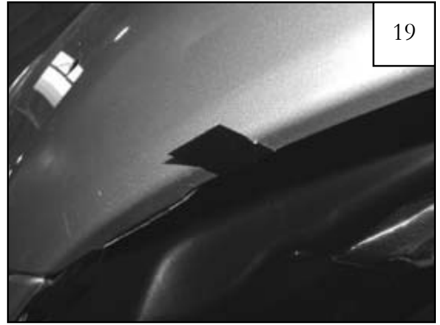
Remove flare from fender. Stick a supplied 1" Black Tab (MT1-0002) over marks made in step 17.
