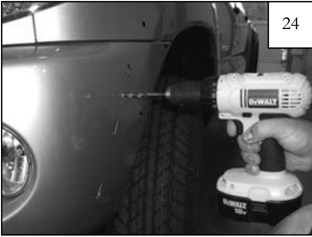
Remove fasteners installed in Step 21-22 and remove flare from fender. Drill at marked places with a 5/16" drill bit
