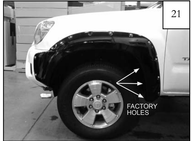
Reposition flare on fender and install three 20mm hex screws (SW1-0036) through holes in flare and into factory holes
