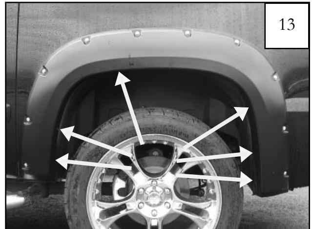
Screw locations.
