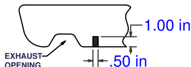
REAR BUMPER FASCIA TRIM DIAGRAM
