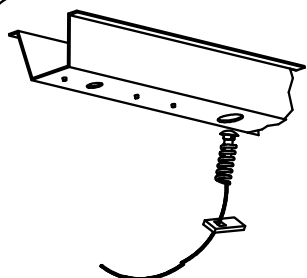
REVERSE FISHWIRE (FOR 1/2" FASTENERS)
