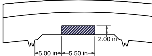
TRIM DIAGRAM
