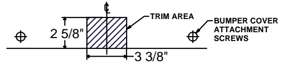
BUMPER COVER TRIM DIAGRAM
