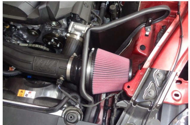
29. Install the clamp (2) on the air filter (1), then install the filter on the filter adapter and tighten the clamp.
