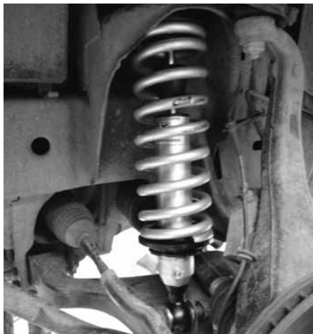
Fig. 2: Driver side
