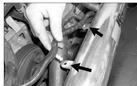
24. Insert the wire harness push clips into the tabs on the K&N intake tube as shown.
