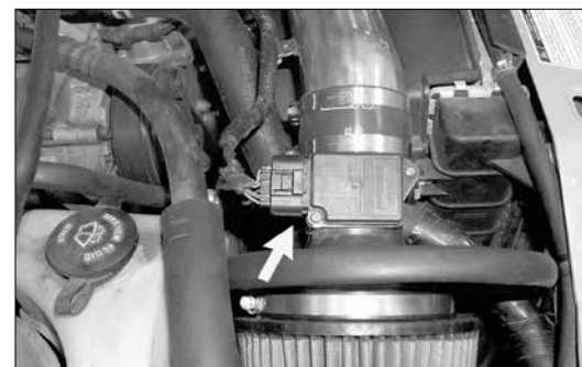
25. Reconnect the mass air sensor electrical connection as shown.
