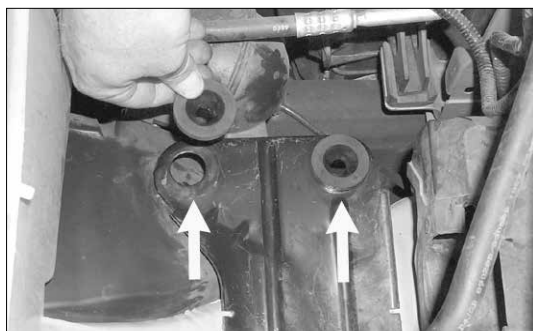
11. Remove the stock grommets from the air cleaner tray.
