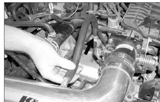
21. Install the provided silicone hose onto the vent on the cam cover, then, connect the other end to the vent on the intake tube as shown.
