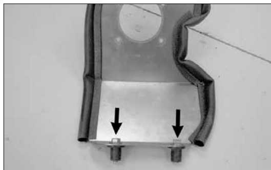
14. Install the hex bolts, washers, and rubber expansion nuts onto the heat shield as shown.
