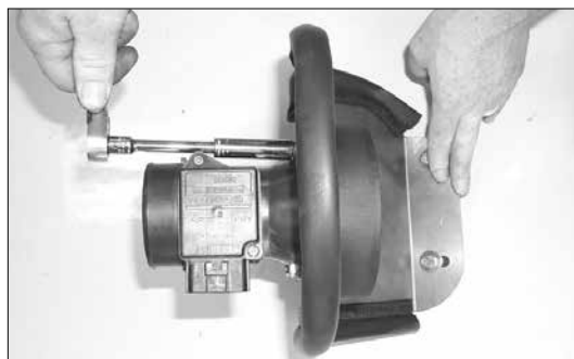
15. Assemble the mass air adapter, gaskets, heat shield and stock mass air sensor using the provided hardware as shown.
