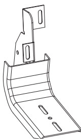
Support (M-1879) X3
