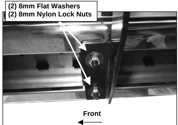
(Fig 10) Attach Bracket to Running Board
