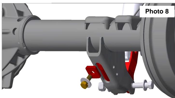
Install Magneride shock relocation brackets.
