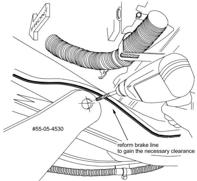
DIAGRAM 4 - DRILLING THE CROSSMEMBER FOR THE "05" BRACKET.
