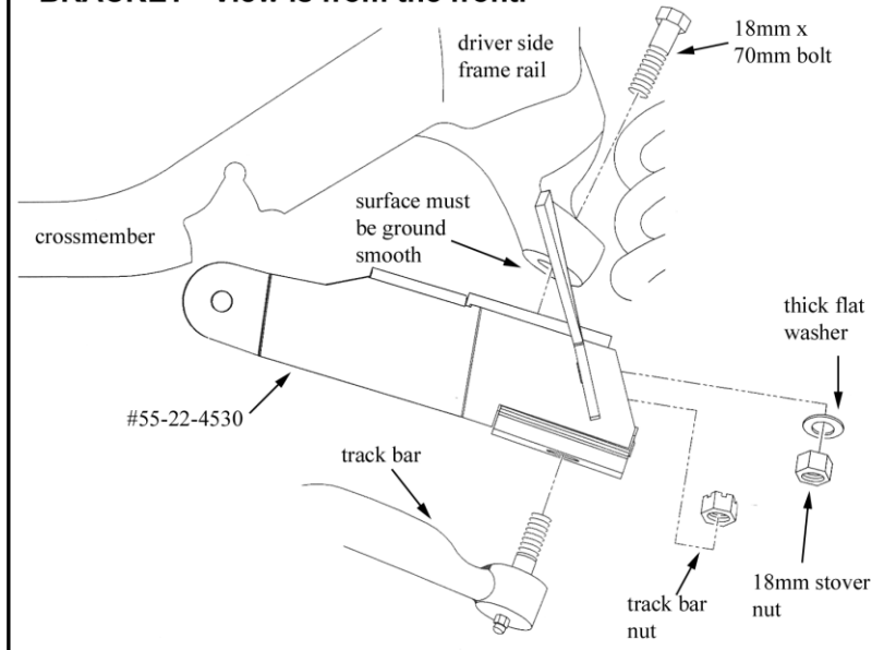
DIAGRAM 5 - INSTALLING THE #55-22-4530 TRACK BAR BRACKET - View is from the front.
