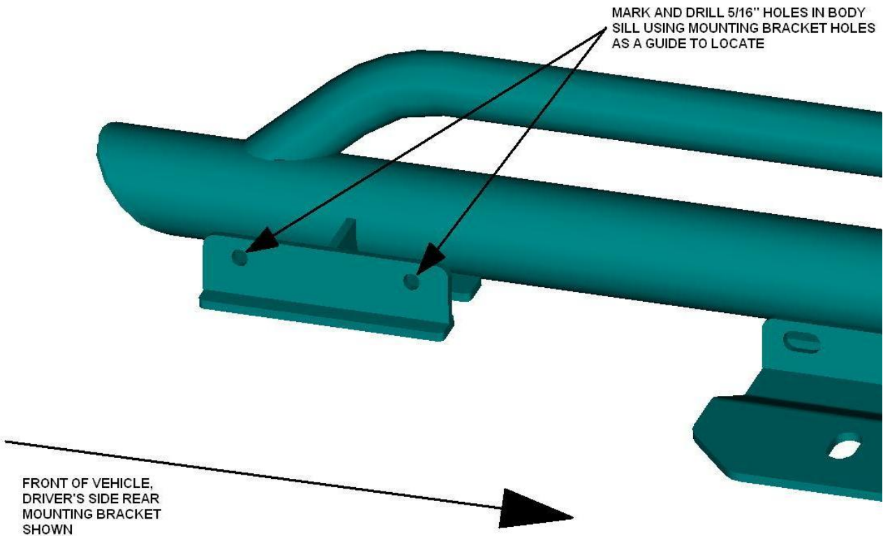
Figure 3: Location of 5/16" holes to be drilled in body sill at rear mounting location
