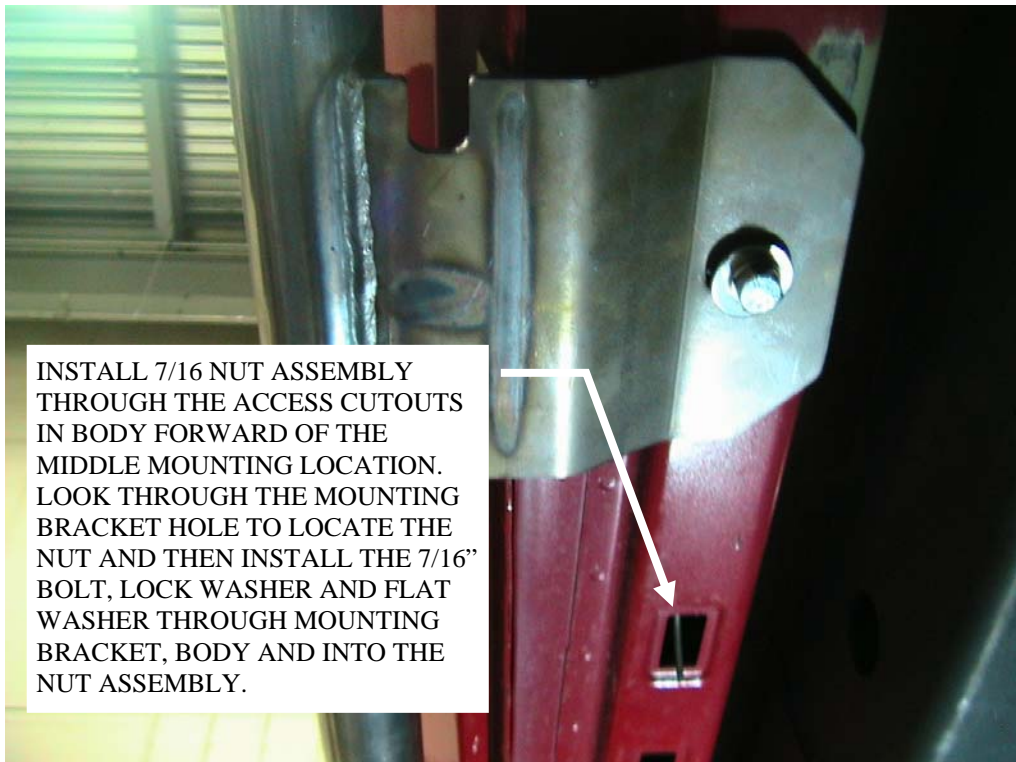
Figure 6: Underside of body middle mounting location
