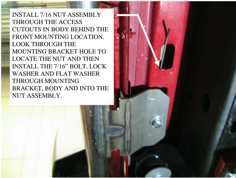
Figure 5: Underside of body front mounting location
