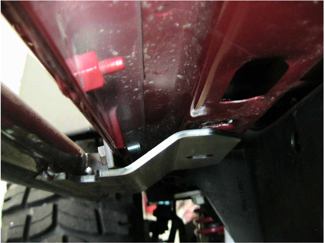
Figure 4: Install four 3/8" bolts and washers through the mounting bracket and then the body sill. Install two 5/16" bolts and washers through the mounting bracket and the two previously drilled holes in rear mounting bracket.
