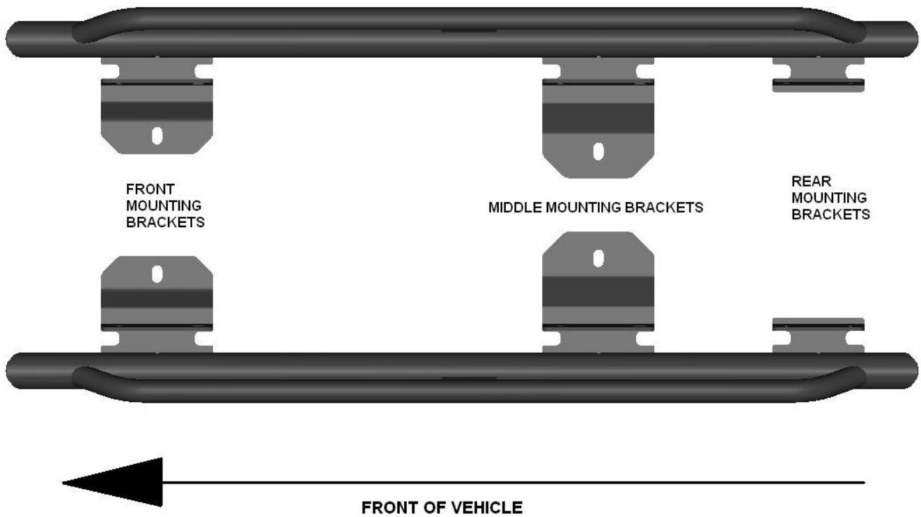
Figure 2: Identifying the Left and Right Rock Sliders
