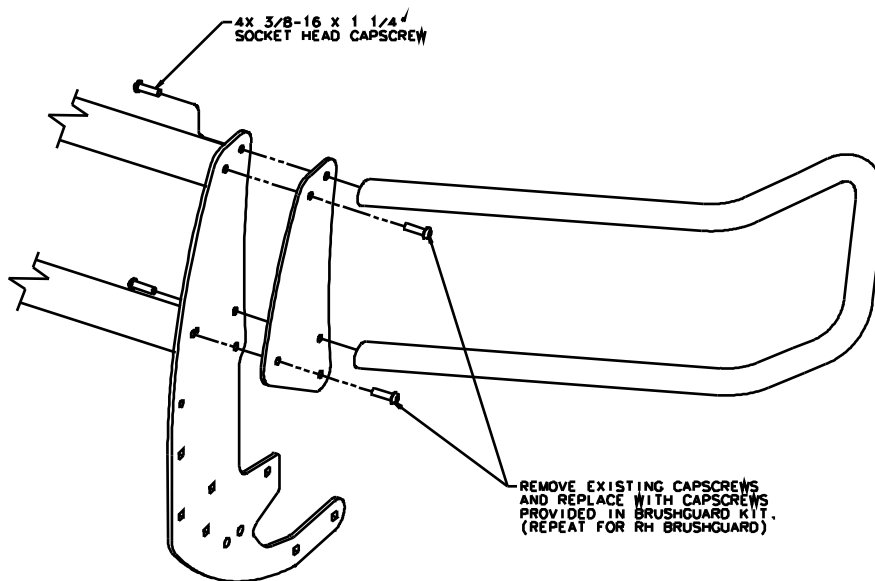
FIGURE 2 LH Brush Guard (Black Kit – one piece)
